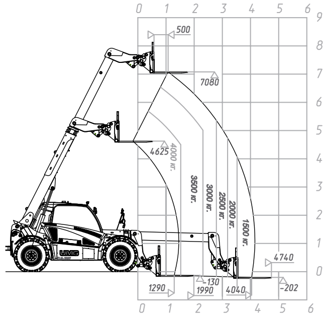
TLH-4007-12 (AG) Floating adjustable pallet fork
