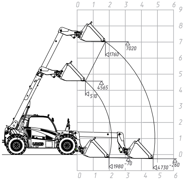
TLH-3507-12 (AG), TLH-4007-12 (AG) Light material bucket
