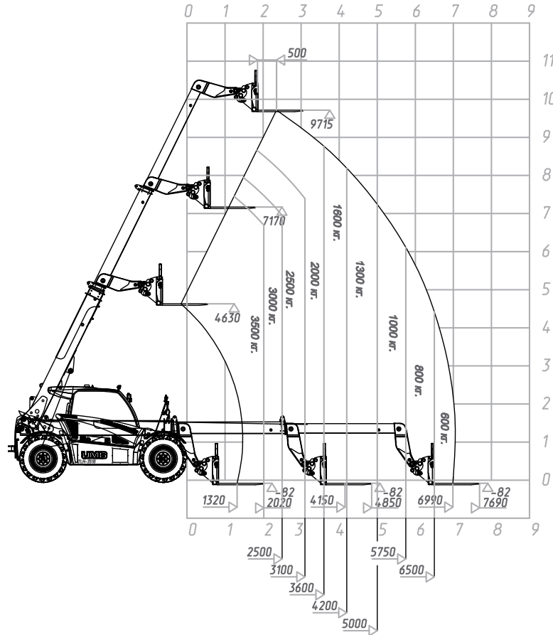
TLH-3510 (AG) Floating adjustable pallet fork
