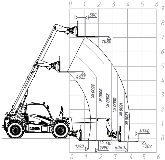
TLH-3507-12 (AG) Floating adjustable pallet fork
